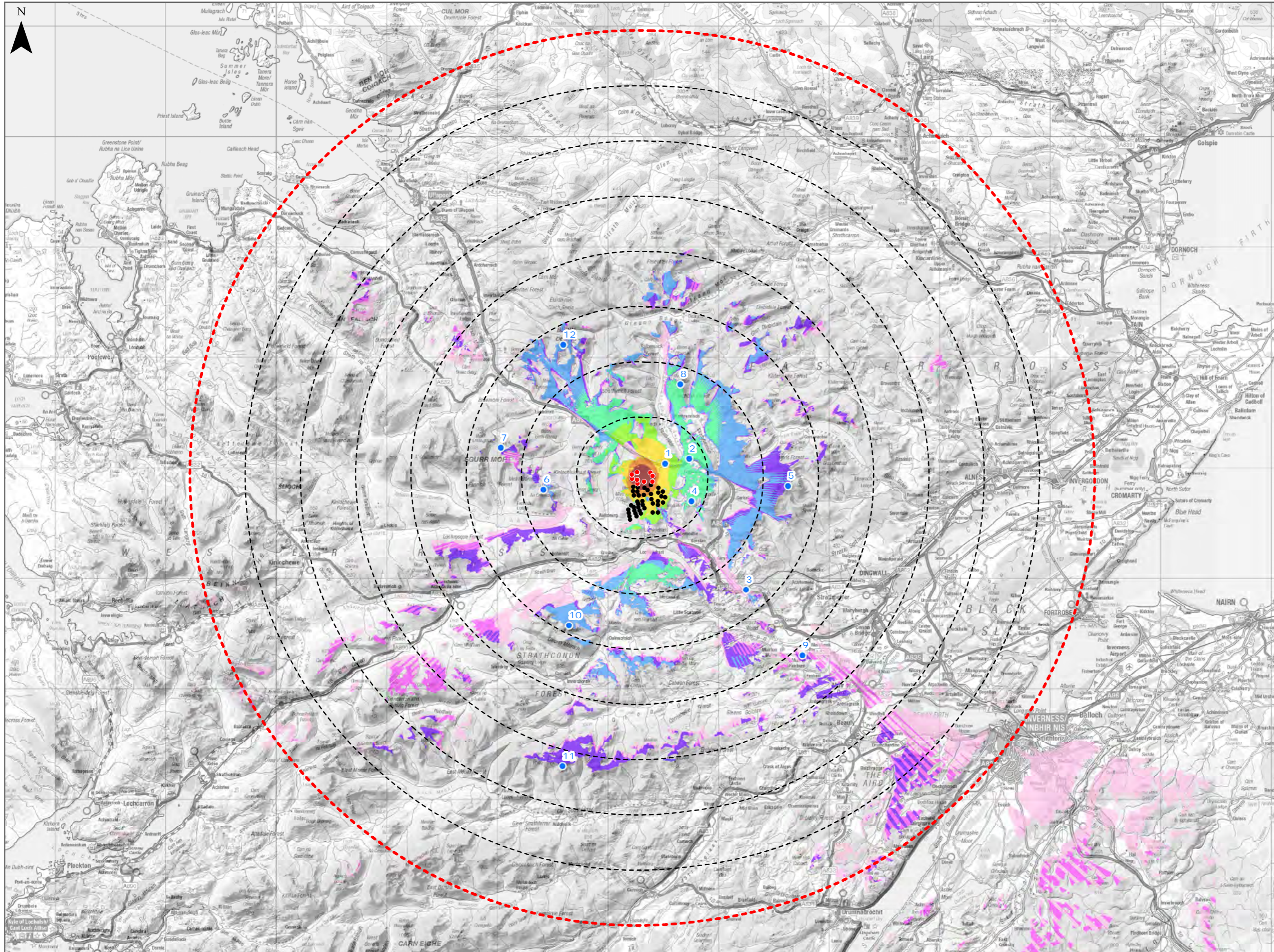
Figure 9.8a: Horizontal Angle ZTV (40km)
